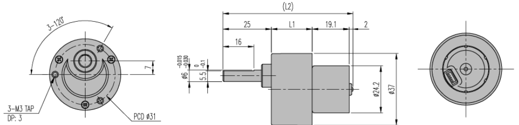
GEARHEAD LENGTH
